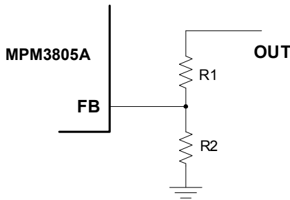
Figure 2: Feedback Network
