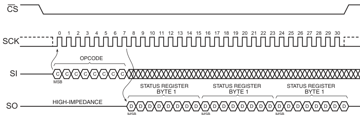
Figure 27. Read Status Register 1
