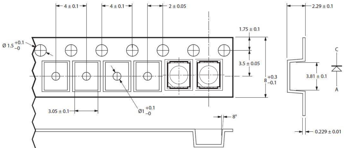
Figure 11. Tape dimensions.
