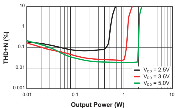
THD+N vs. Output Power (f = 1kHz; R L = 4Ω; Gain = 6dB)
