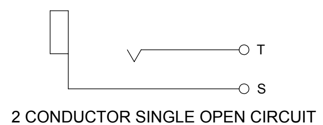
SN70C11
