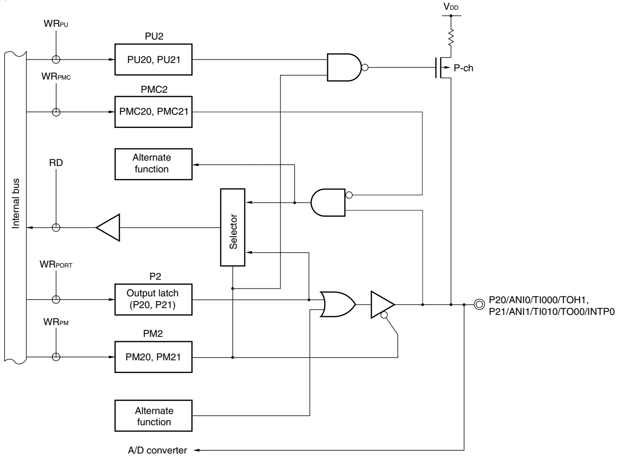
Figure 4-2. Block Diagram of P20 and P21 (1/2)
