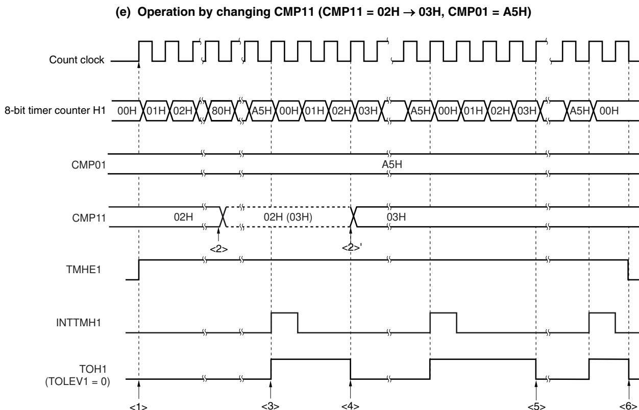
Figure 7-10. Operation Timing in PWM Output Mode (4/4)
