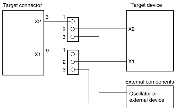
Figure 17-5. Circuit Connection for the Case Where X1 and X2 Pins Are Used in Target System
