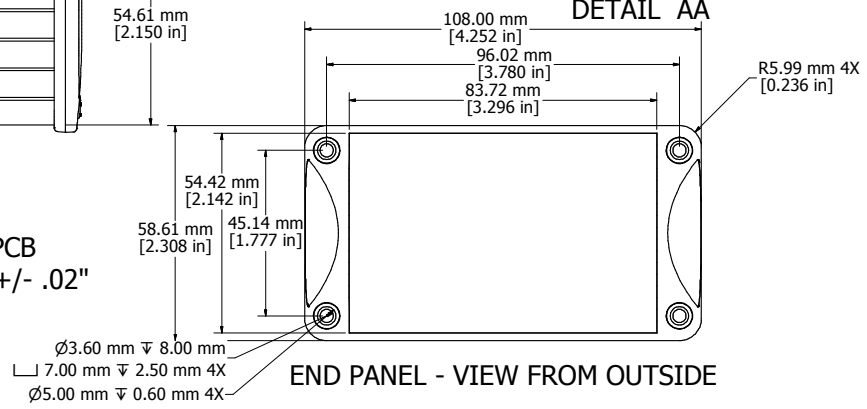
DETAIL AA
