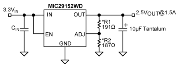
Adjustable Output Voltage
