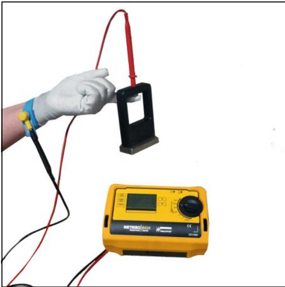
The Model 15 Glove Probe testing. Resistance meter is not included.
