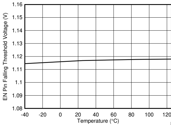
Figure 7-9. EN Pin Threshold Falling vs Temperature
