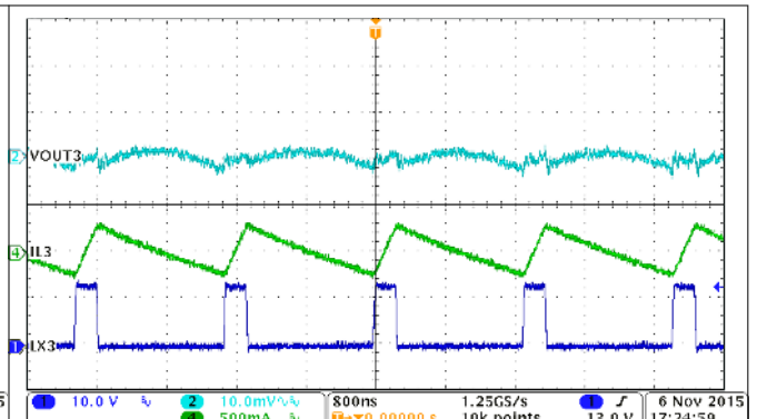
Figure 9-22. Buck3, FCC Mode, Iout = 0 A
