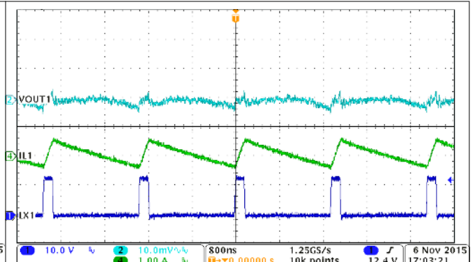
Figure 9-16. Buck1, FCC Mode, Iout = 0 A
