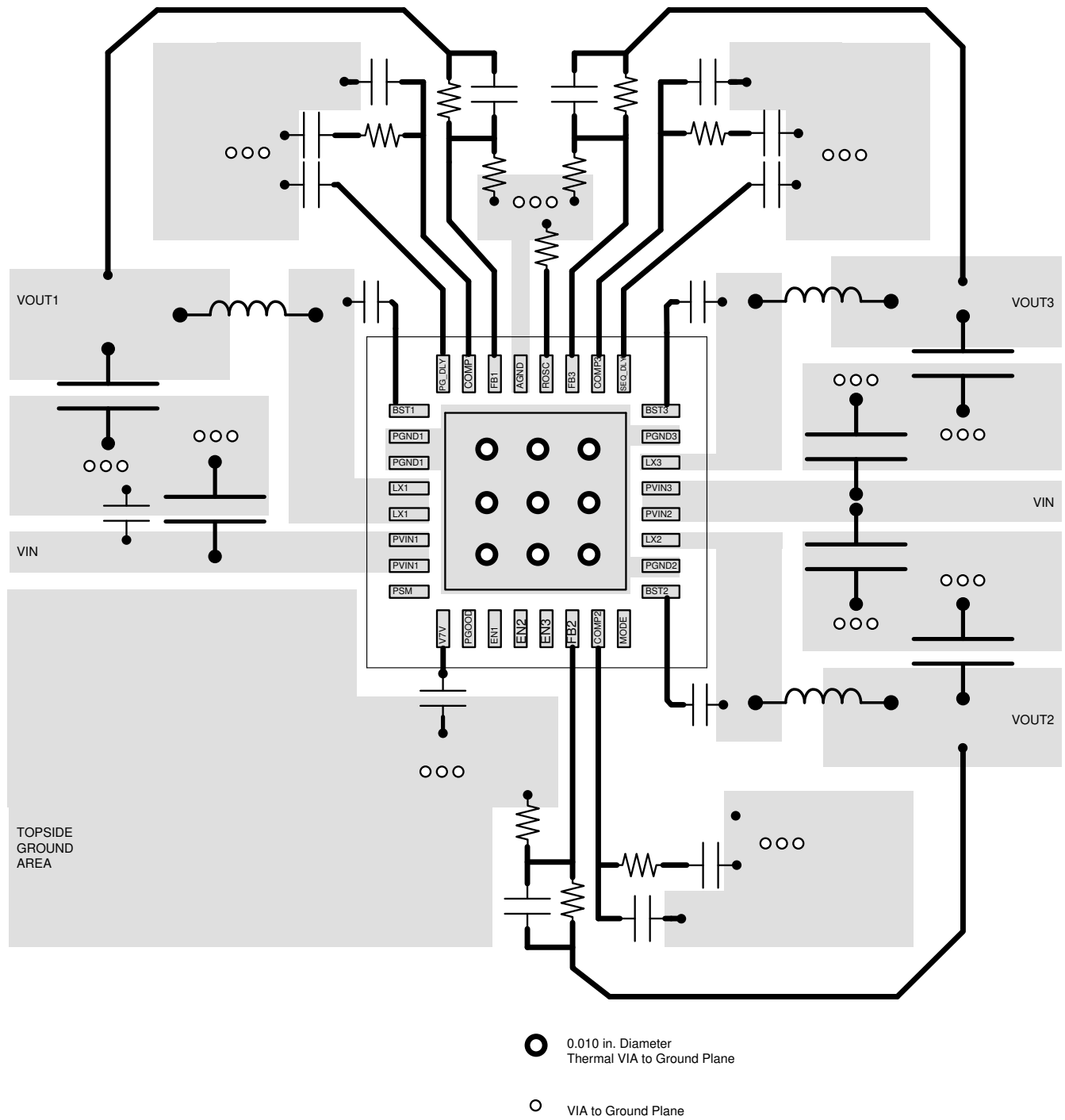
Figure 9-41. PCB Layout
