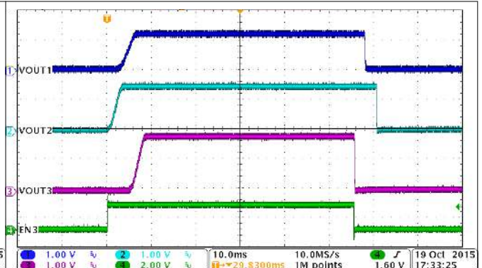
Figure 9-34. Automatic Power Sequencing, MODE = LOW, EN1 = LOW, EN2 = HIGH
