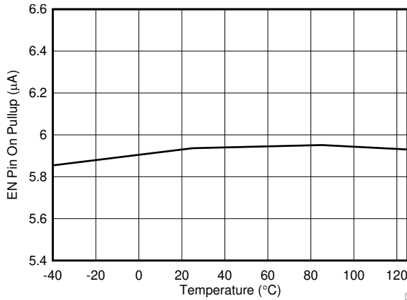
Figure 7-7. EN Pin Pullup Current vs Temperature, EN = 1.5 V
