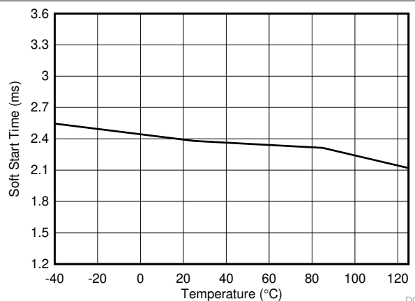
Figure 7-12. Soft-Start Time vs Temperature
