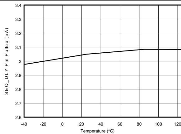
Figure 7-11. SEQ_DLY Pin Pullup Current vs Temperature, PG_DLY = 0.5 V
