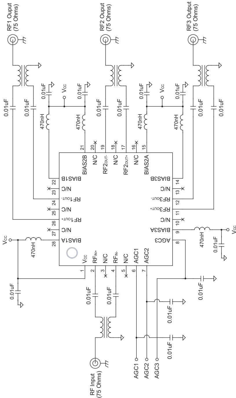
Figure 3: Application Circuit
