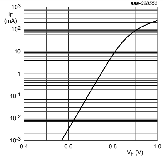
Fig. 4. Forward current as a function of forward voltage; typical values (BZX384-A7V5)
