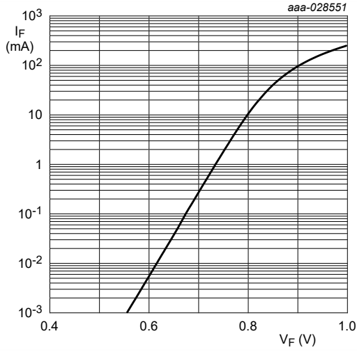
Fig. 3. Forward current as a function of forward voltage; typical values (BZX384-A6V8)
