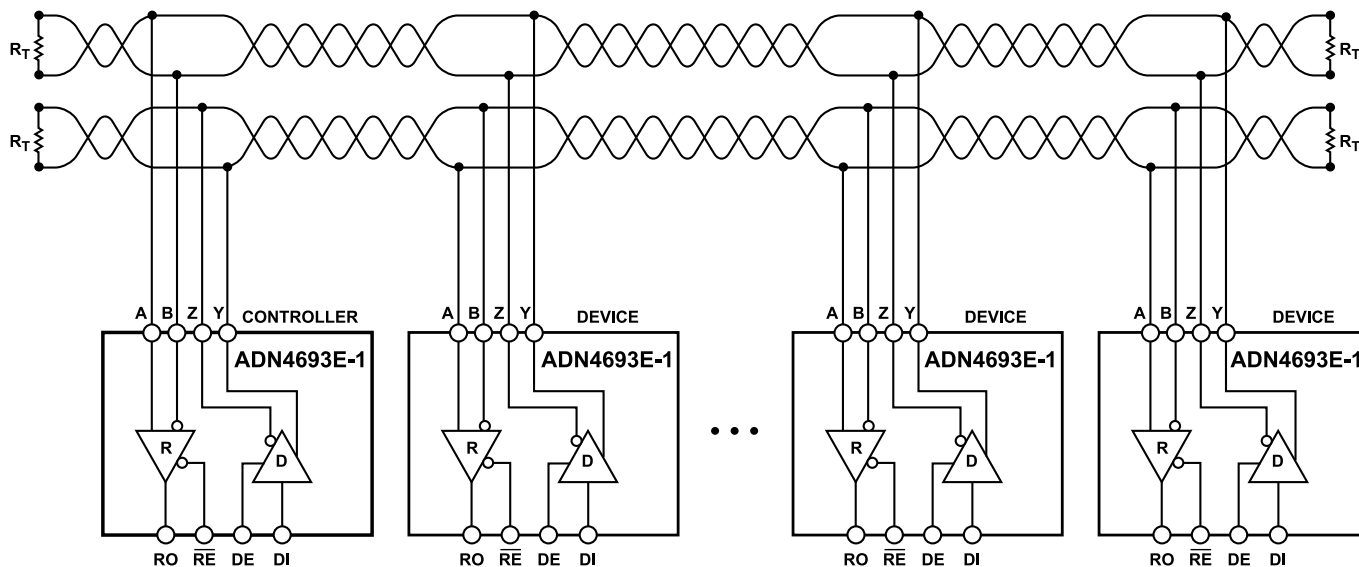
Figure 38. ADN4693E-1 Typical Full-Duplex M-LVDS Controller/Device Network (Type 1 Receivers)
