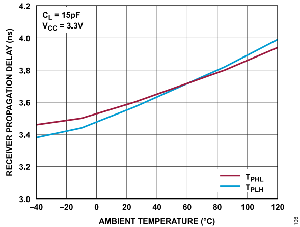
Figure 10. Receiver Propagation Delay vs. Ambient Temperature (Clock Frequency = 100 MHz, V_{ID} = 300\text{ mV} , V_{IC} = 1.1\text{ V} )
