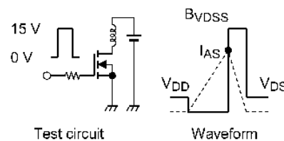
Fig. 8.16 Test Circuit/Waveform
