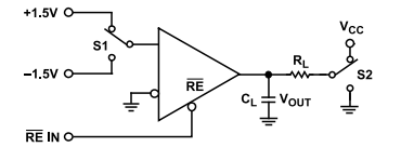
Figure 42. Receiver Propagation Delay/Skew
