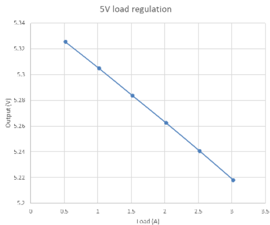
Figure 10. 5 V Regulation
