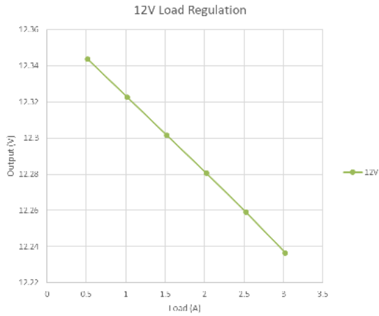
Figure 12. 12 V Regulation
