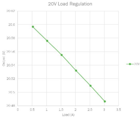
Figure 14. 20 V Regulation
