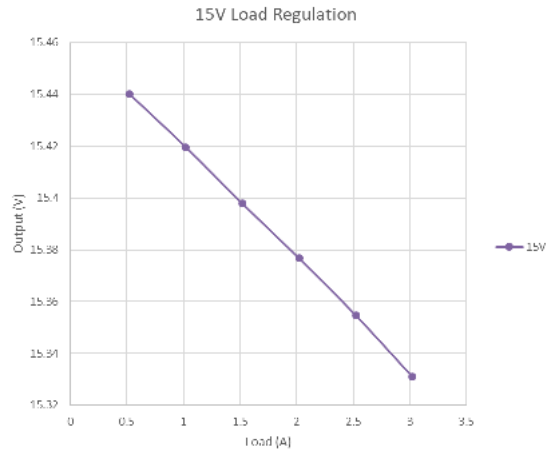
Figure 13. 15 V Regulation
