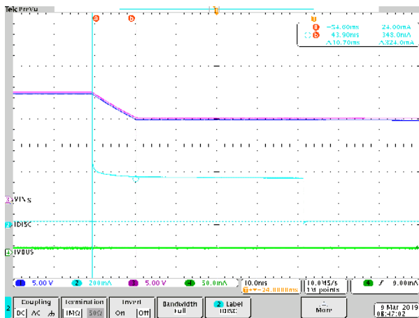
Figure 41. VBUS Discharge, from 20 V to 15 V, without a Load
