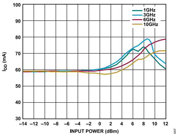
Figure 57. I_{DQ} vs. Input Power for Various Frequencies, V_{DD} = 5\text{ V} , R_{BIAS} = 1.47\text{ k}\Omega
