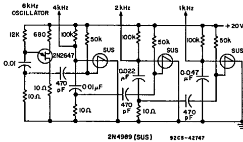
Fig. 21—Frequency divider circuit (with transient-free output).
