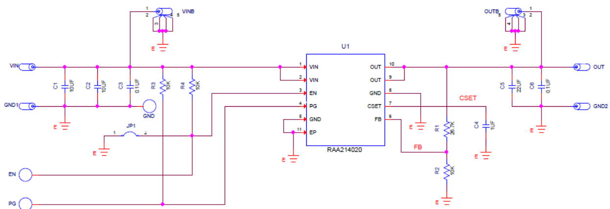
Figure 3. RTKA214020DE0010BU Schematic
