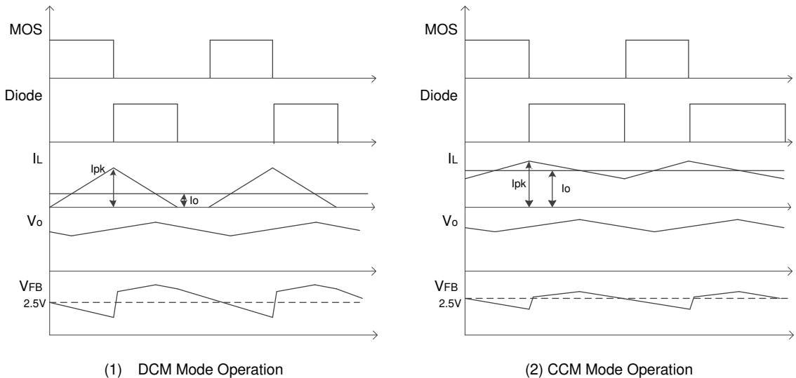
Figure 4. Operation Timing of AL17150-10B
