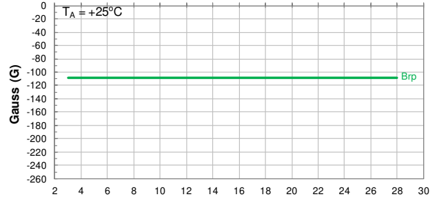
Supply Voltage (V) Switch Release Point Brp vs Supply Voltage
