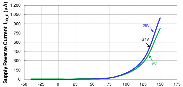
Temperature (°C) Supply Reverse Current vs Temperature
