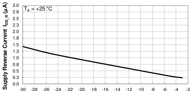
Supply Voltage (V) Supply Reverse Current vs Supply Voltage
