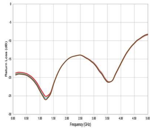
Figure 16. Return Loss: RFC @ 25 °C
