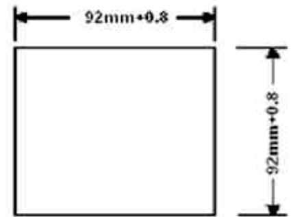
Installation Cutout
