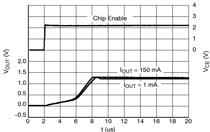
Figure 36. Start-up, 1.2 V Version, V_{\text{IN}} = 2.2 \text{ V}
