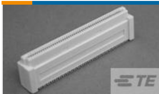
TE Part #6-6123212-0 0.8FH,R13H.5,200,30/Sn,TU
