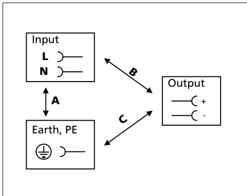
Fig. 17-1 Dielectric strength
