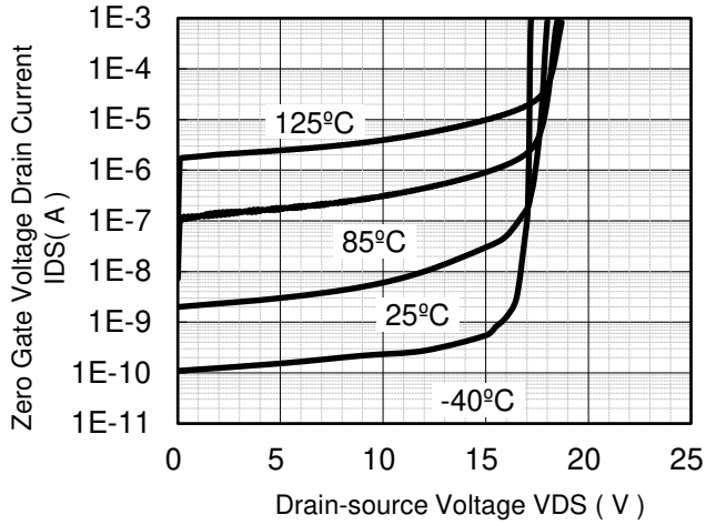
IDS - VDS
