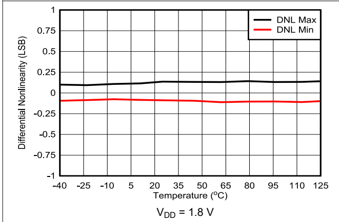
Figure 7-10. Differential Nonlinearity vs Temperature
