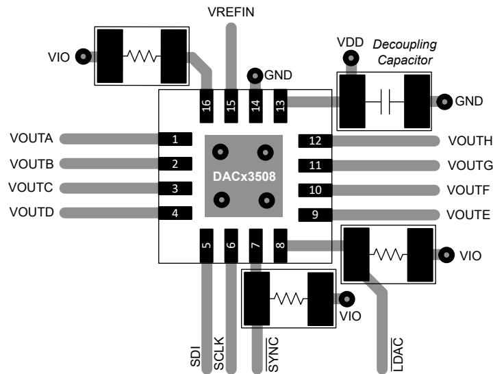
Figure 11-1. Layout Example
