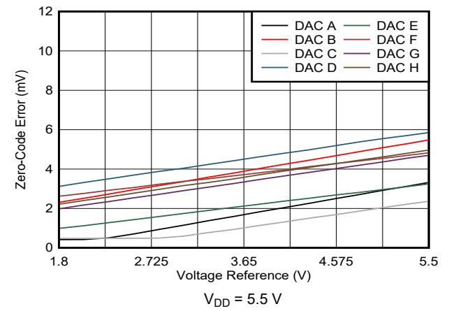
Figure 7-23. Zero-Code Error vs Voltage Reference
