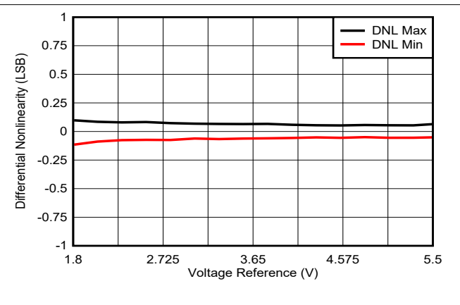
Figure 7-13. Differential Nonlinearity vs Voltage Reference
