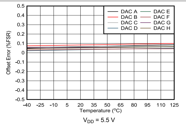
Figure 7-25. Offset Error vs Temperature
