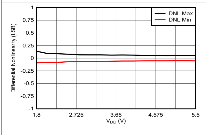
Figure 7-12. Differential Nonlinearity vs Supply Voltage
