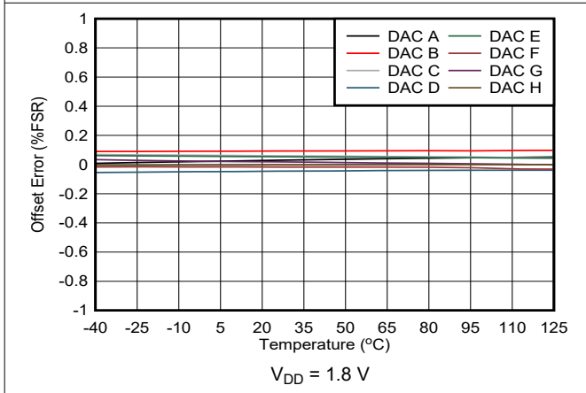
Figure 7-24. Offset Error vs Temperature
