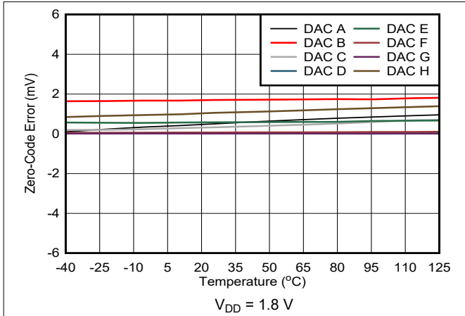
Figure 7-20. Zero-Code Error vs Temperature
