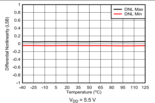
Figure 7-11. Differential Nonlinearity vs Temperature
