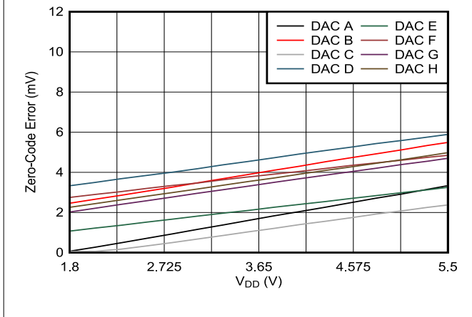
Figure 7-22. Zero-Code Error vs Supply Voltage
