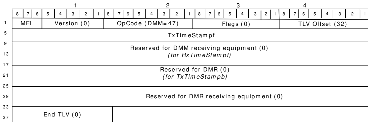
Figure 66 • Y.1731 DMM PDU Format
