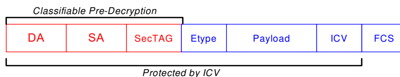
Figure 25 • Single-Tagged Ethernet
