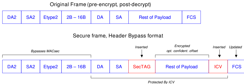
Figure 41 • EoMPLS Header Bypass Format
