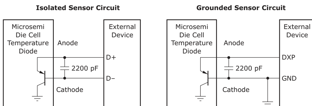
Figure 118 • Thermal Diode
