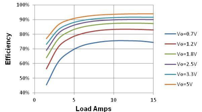
Figure 6. Efficiency vs. Load. V_{in} = 12\text{V} , F_{sw} = 1\text{MHz}
