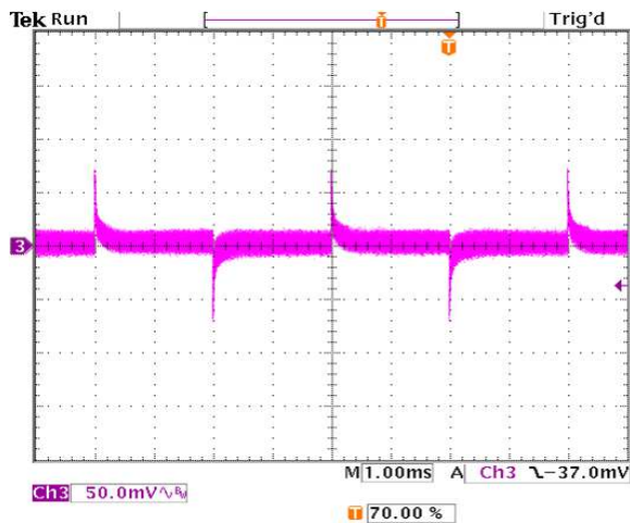
Figure 50. Transient Response with Regulation set to 0.0 mV/A.
