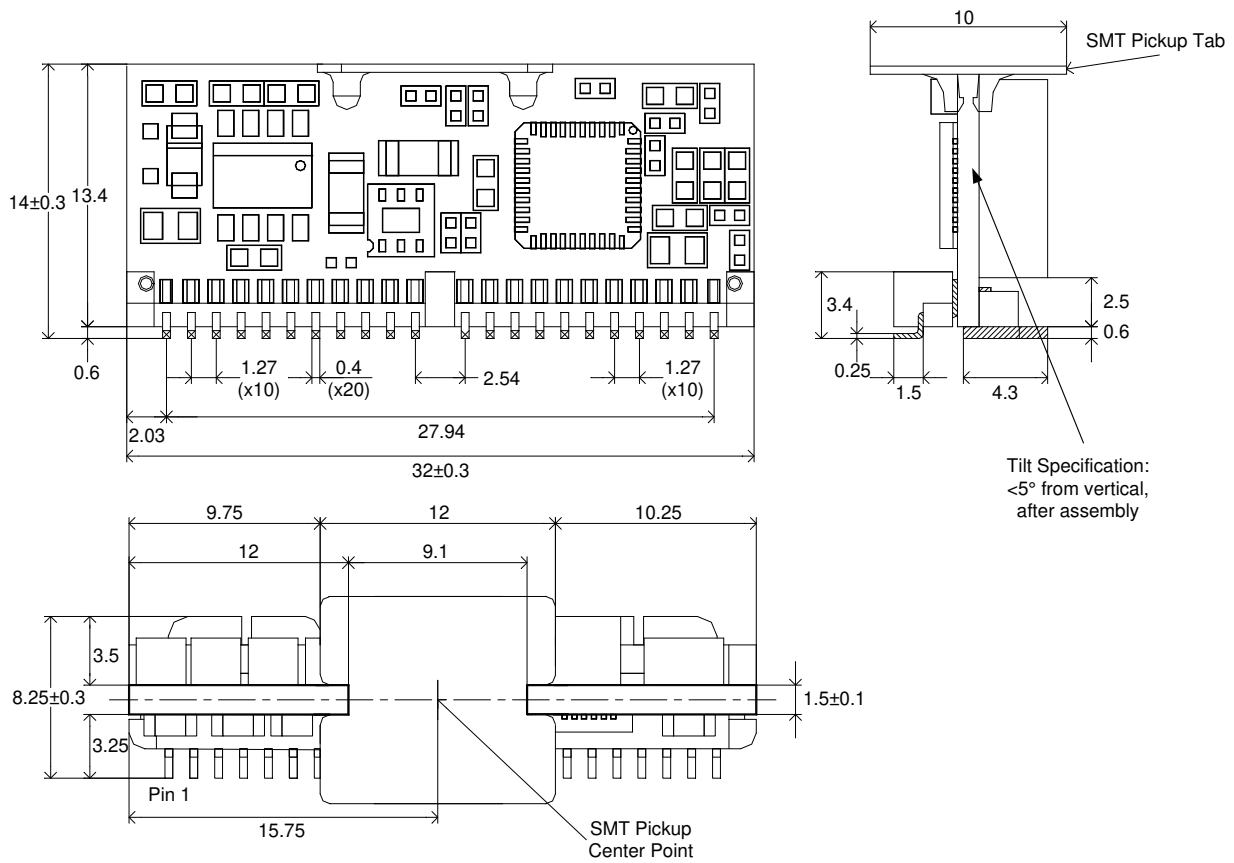
Figure 58 Mechanical Drawing
