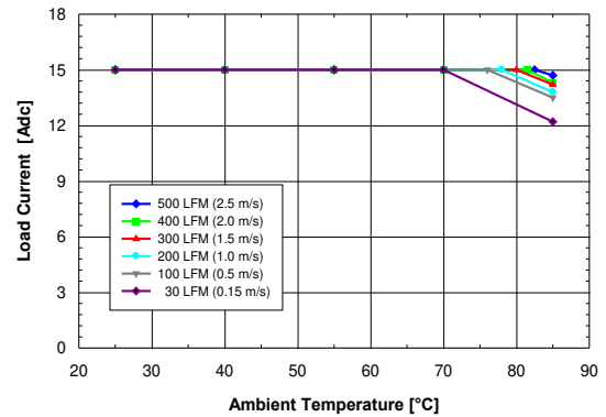
Figure 4. Available output current vs. ambient air temperature and airflow rates for converter DP7115G mounted horizontally with air flowing from input to output, MOSFET temperature 120^\circ\text{C} , V_{in} = 12\text{ V} , V_{out} = 5\text{ V} , and F_{sw} = 1\text{MHz}
