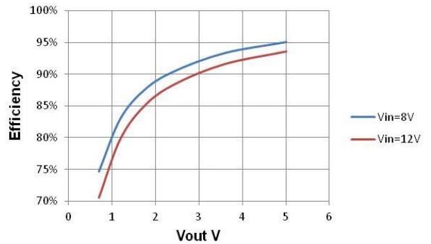
Figure 10 Efficiency vs Vout, Fsw=1MHz
