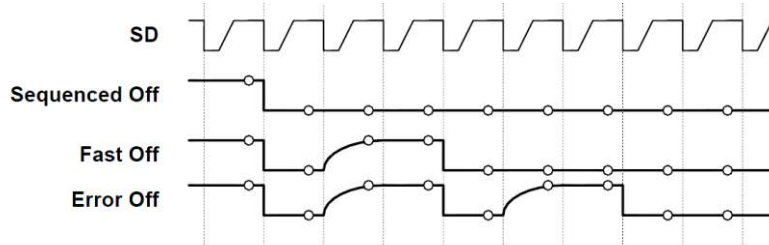
Figure 42. OK Severity Encoding Waveforms
