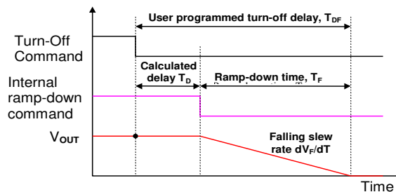
Figure 20. Relationship between Turn-Off Delay and Falling Slew Rate
