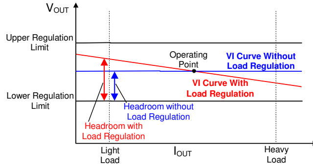
Figure 15. Optimal Voltage Positioning Concept
