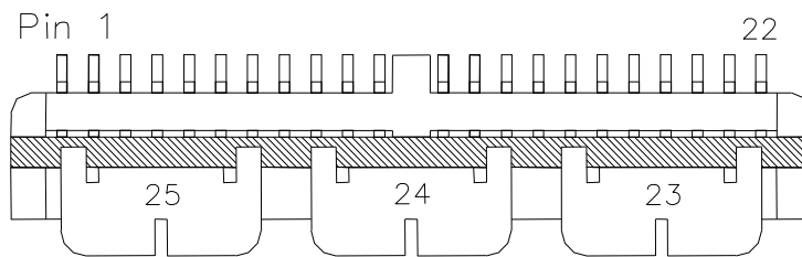
Figure 59. Pinout Diagram (Bottom View)
