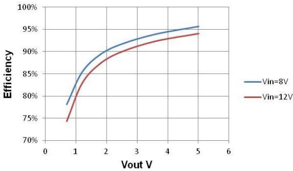
Figure 9 Efficiency vs Vout, Fsw=500KHz
