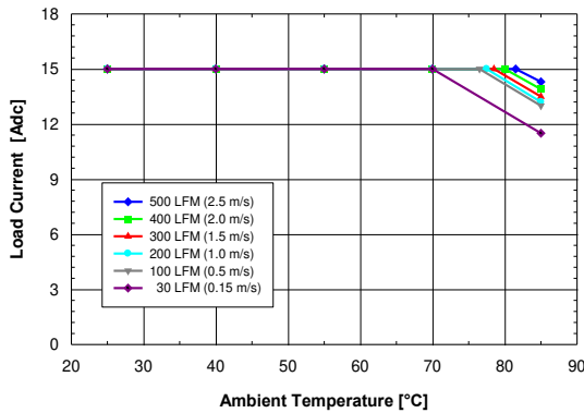
Figure 3. Available output current vs. ambient air temperature and airflow rates for converter DP7115G mounted horizontally with air flowing from input to output, MOSFET temperature 120^\circ\text{C} , V_{in} = 12\text{ V} , V_{out} = 5\text{ V} , and F_{sw} = 500\text{KHz}
