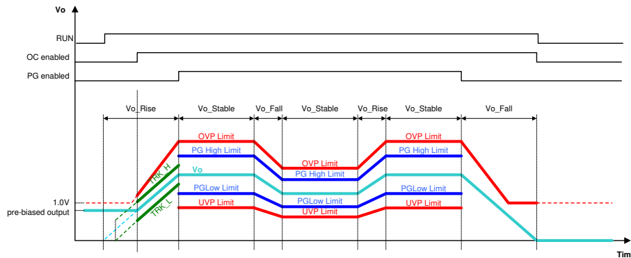
Figure 32. Protection Enable Conditions
