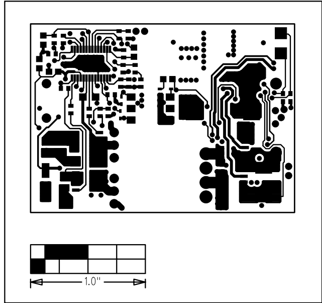
Figure 11. MAX5058 EV Kit PC Board Layout—Component Side
