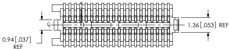
FIG 1 ST5-20-1.00-X-D-P-TR SHOWN
