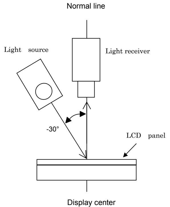
Figure 7-3 Response time
