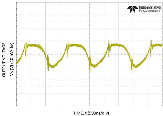
Figure 33. Typical output ripple and noise ( C_o=2x47\mu F ceramic, V_{IN} = 12V , I_o = I_{o,max} ).
