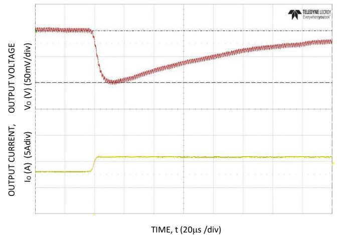
Figure 34. Transient Response to Dynamic Load Change from 50% to 100% at 12Vin, C_{out}=5x47\mu F , C_{Tune}=1800pF , R_{Tune}=300\Omega
