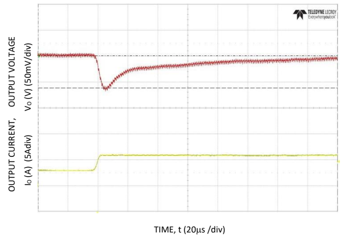
Figure 28. Transient Response to Dynamic Load Change from 50% to 100% at 12Vin, Cout=5x47µF, CTune=1800pF, RTune=300
