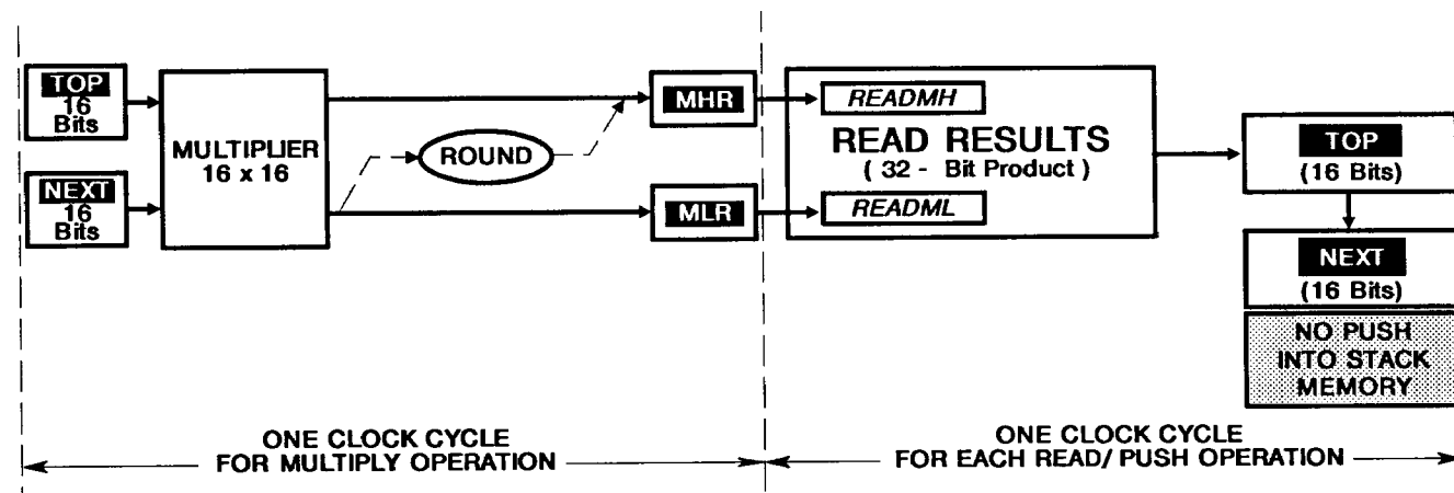
FIGURE 16. MULTIPLIER OPERATION
