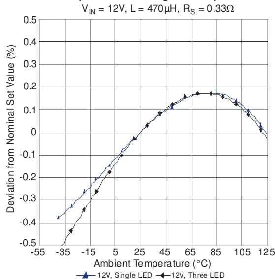
Output Current Change vs. Temperature V IN = 12V, L = 470 μH, R S = 0.33 Ω
