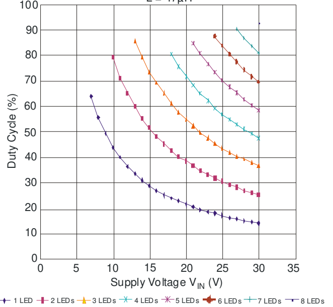
ZXLD1360 Duty Cycle L = 47μH
