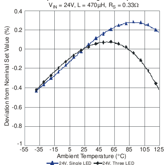
Output Current Change vs. Temperature V IN = 24V, L = 470 μH, R S = 0.33 Ω
