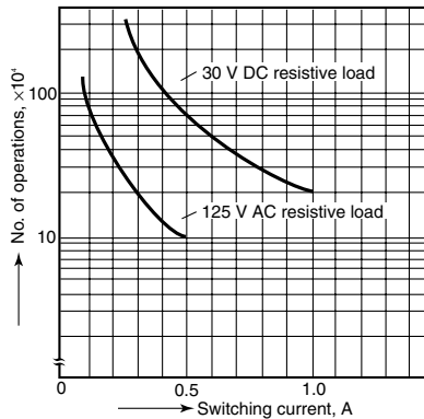
2. Life curve
