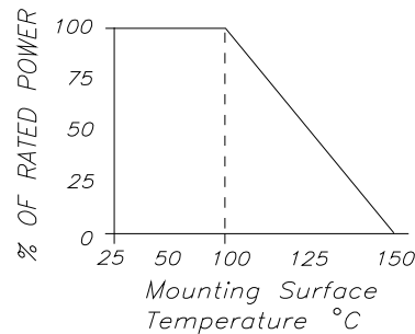
DERATING CURVE:
