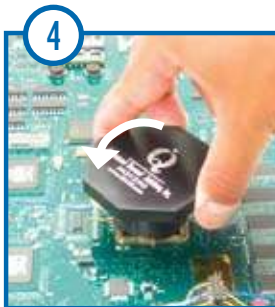
4 Position the Knob Tool with Frame Clip over the component, rotate 45° counter-clockwise releasing the Frame Clip
