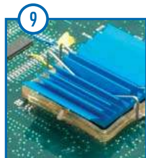
9 Inspect the installation. Double check to make sure the Heat Sink is securely attached.
