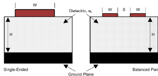
Figure 24. Microstrip Topology
