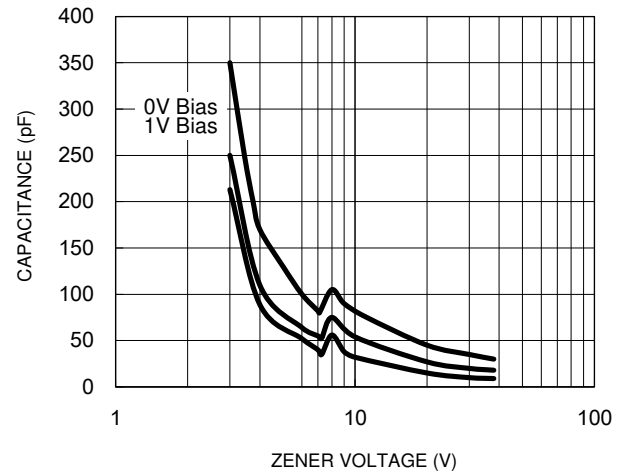
Fig.6 Typical Capacitance
