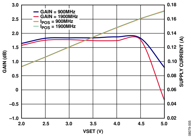
Figure 5. Power Conversion Gain and Supply Current vs. VSET
