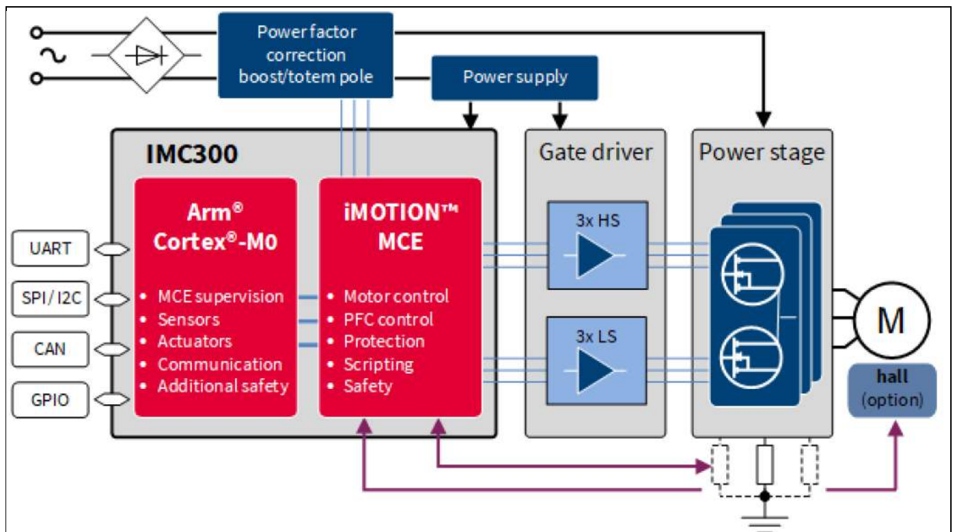
Figure 2 Typical application block diagram using IMC302A-F064
