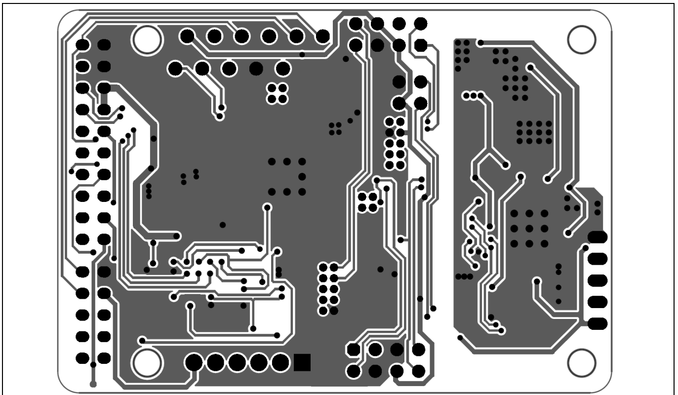
Figure 30 Bottom layer routing of the EVAL-M3-302F
