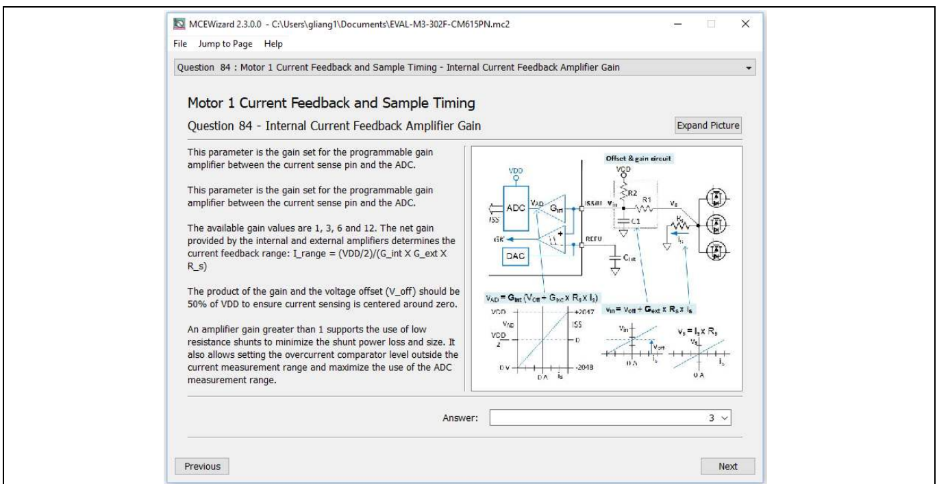
Figure 15 Internal current-feedback amplifier-gain configuration
