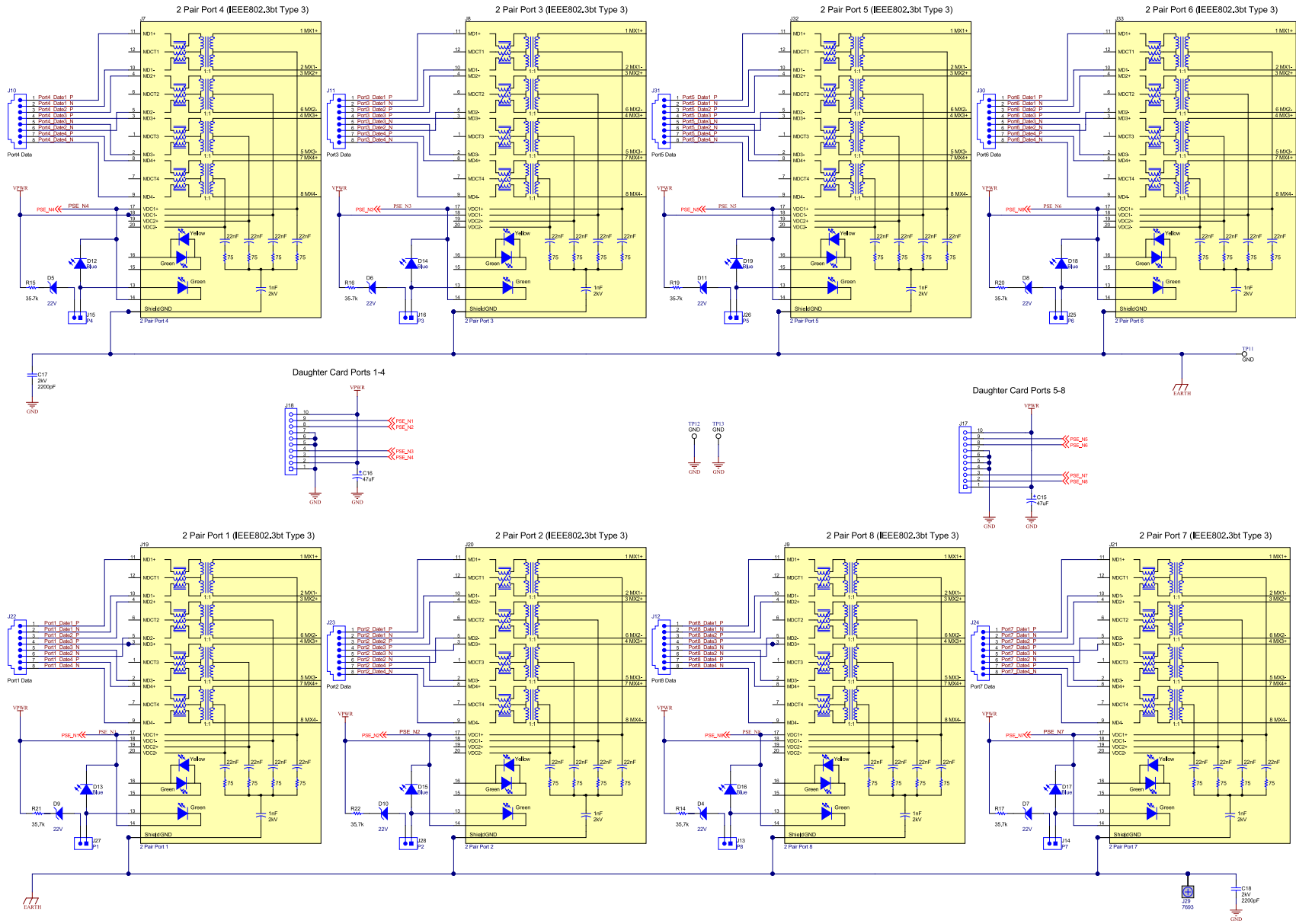
Figure 14. BOOST-PSEMTHR8-097 (Motherboard) Schematic: Power Ports
