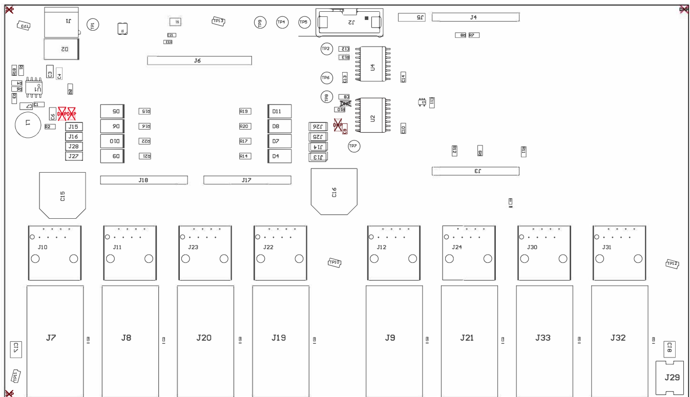
Figure 16. BOOST-PSEMTHR8-097 (Motherboard) Top Side Assembly
