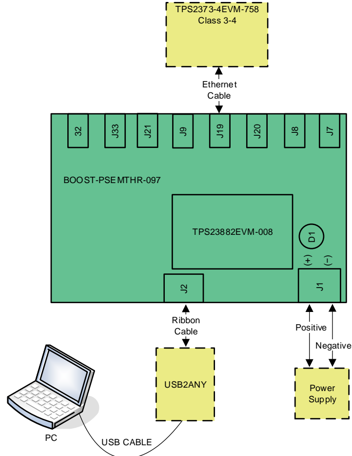
Figure 2. Basic Setup Using USB2ANY
