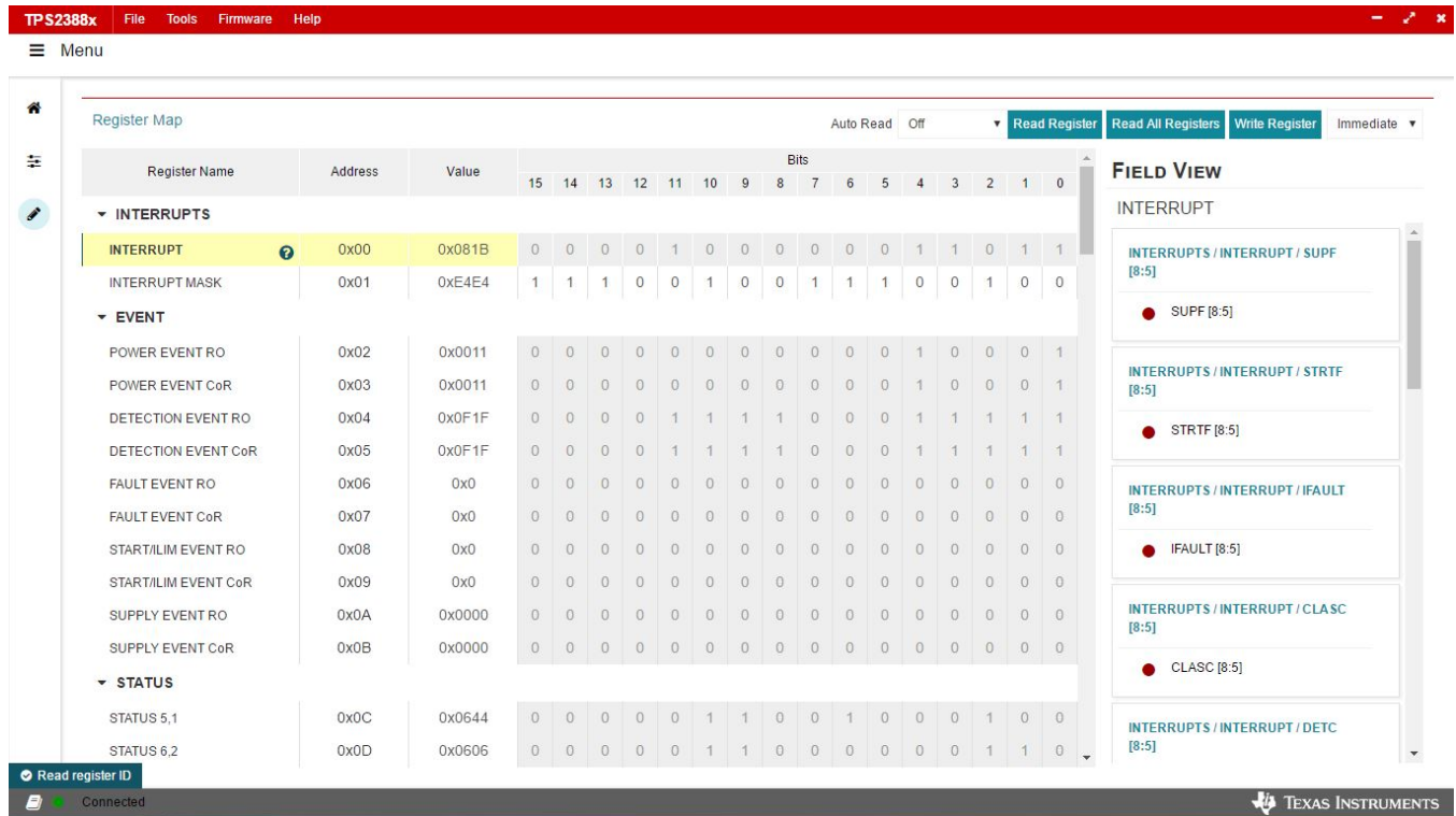
Figure 8. Register Map
