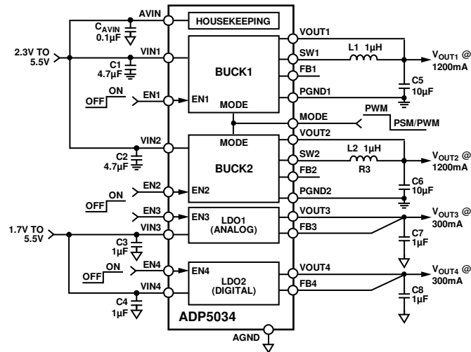
Figure 53. ADP5034 Fixed Output Voltages with Enable Pins
