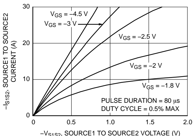
Figure 2. On-Region Characteristics
