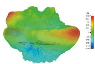
Typical 3D Pattern Side -5400MHz
