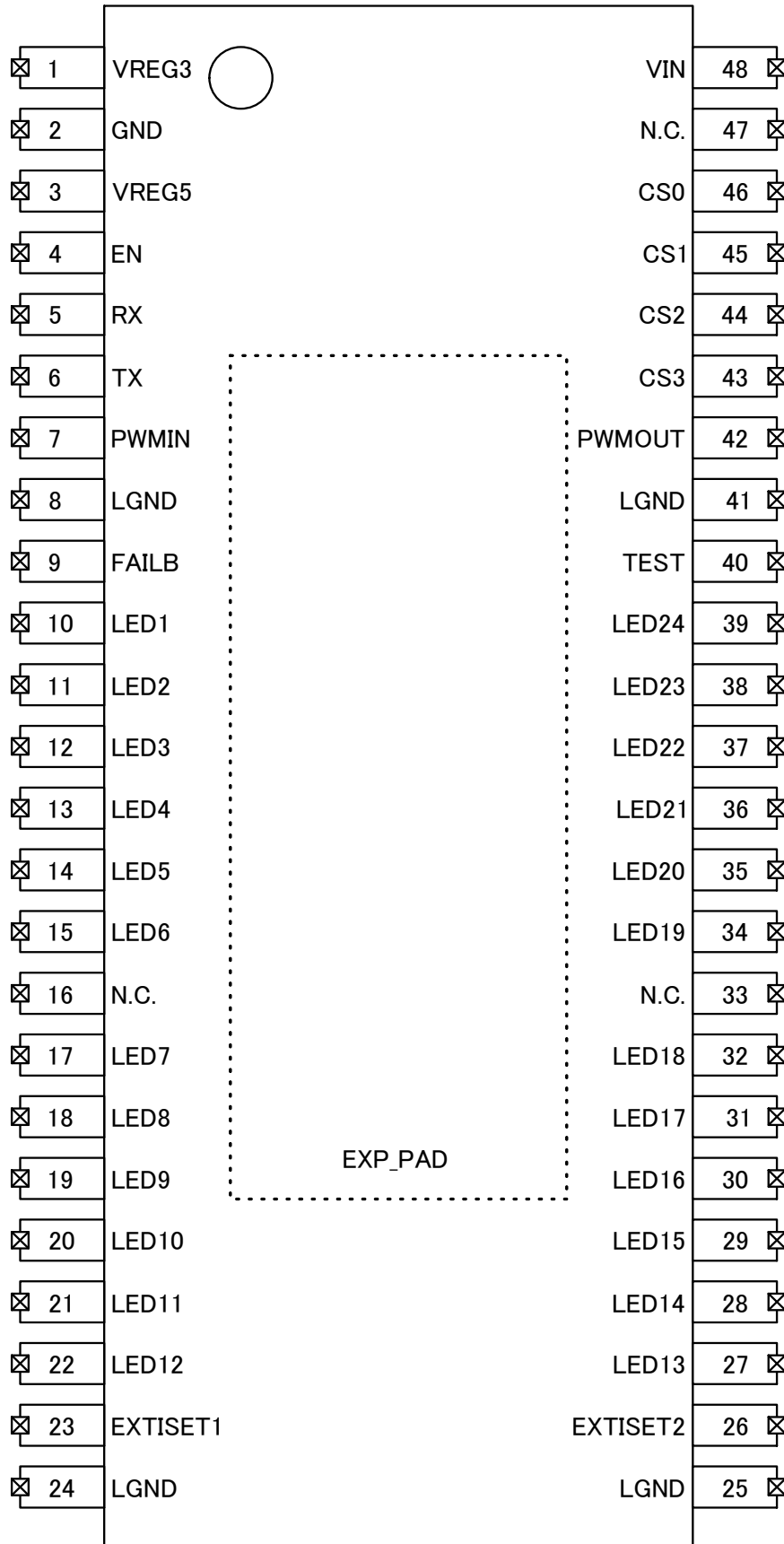
Figure 2. Pin Configuration
