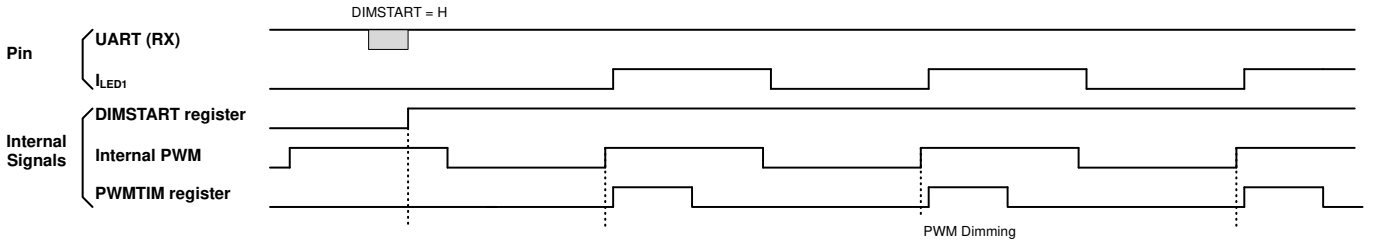
Figure 48. PWMFREQ = 0
