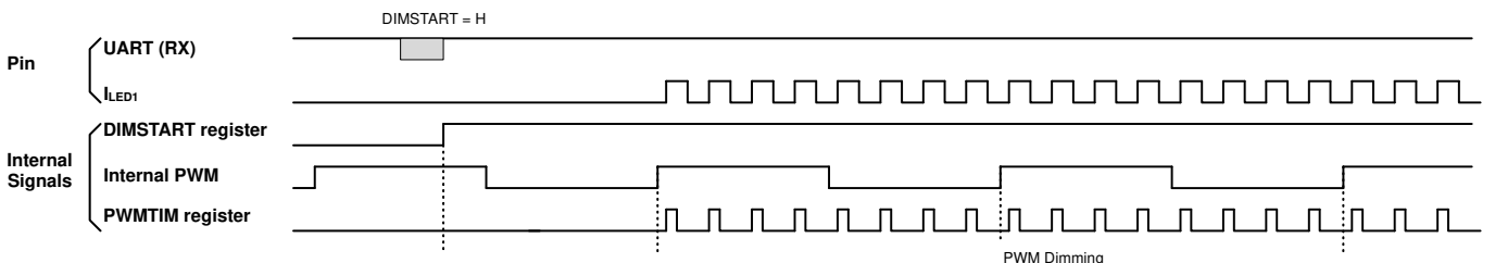
Figure 51. PWMFREQ = 3
