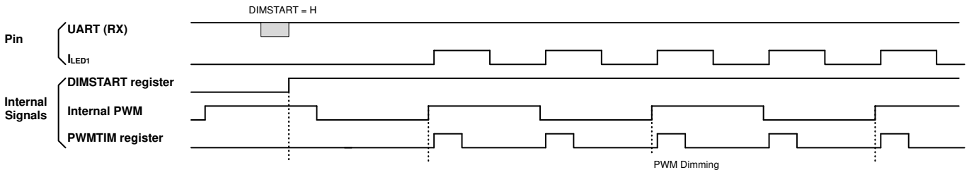
Figure 49. PWMFREQ = 1
