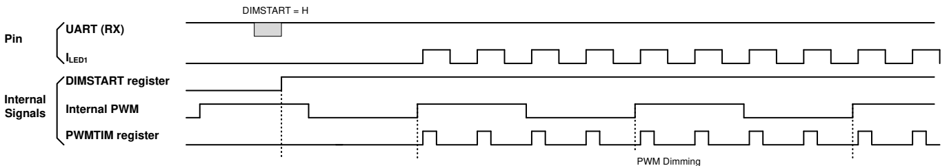
Figure 50. PWMFREQ = 2
