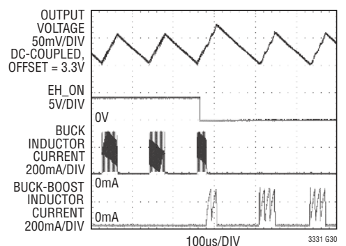
Prioritizer Buck to Buck-Boost Transition
