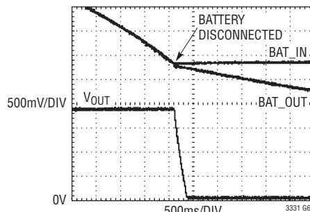
Battery Connect Transient
