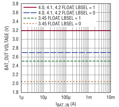
Battery Disconnect Voltage at BAT_OUT vs I_{BAT\_IN}
