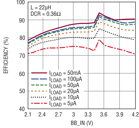
Buck-Boost Efficiency vs BB_IN for V_{OUT} = 3.3\text{V} , 250mA I_{PEAK} Setting
