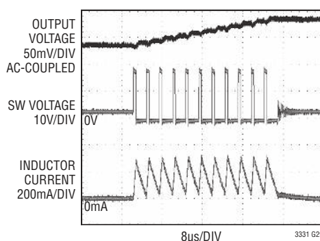
Buck Switching Waveforms
