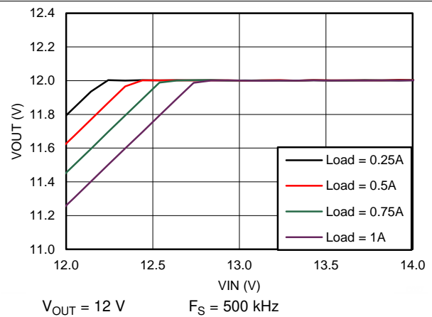
Figure 74. Dropout Curve
