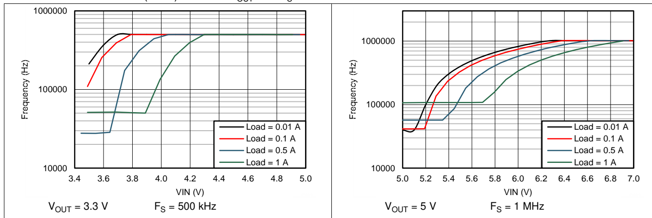
Figure 19. Switching Frequency vs V_{IN} in Dropout Operation
